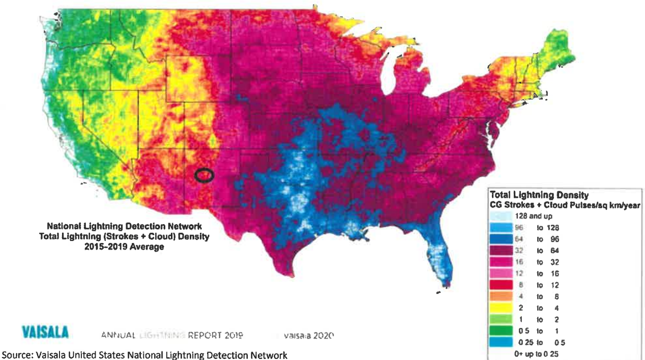
Figure 5-4: Lightning Flash Density in the United States
