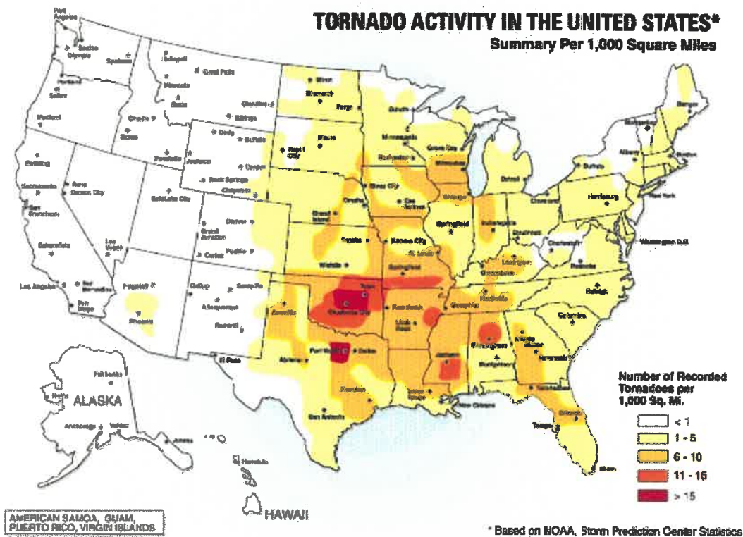
Figure 5-7: Tornado Activity in the United States
